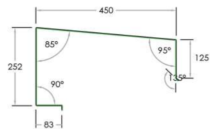
SECTION A Scale 1: 10
