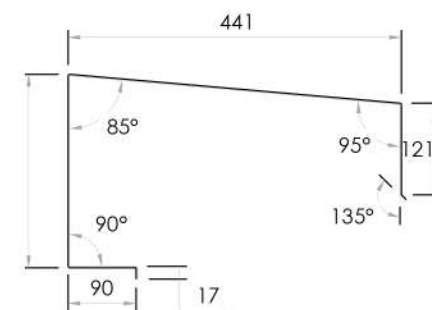
SECTION A Scale 1: 10
